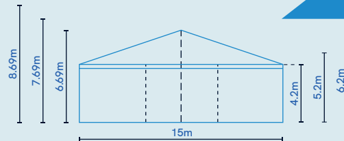
15m Wide
