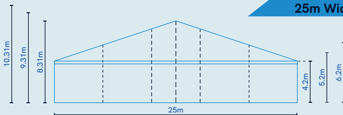
25m Wide
