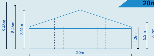
20m Wide
